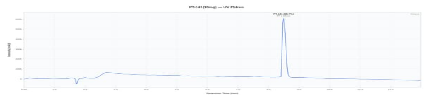
PT-141 10mg - PT141-297: UV Chromatogram
