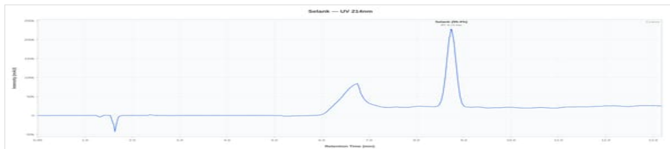
Selank 10mg - SLK10-318: UV Chromatogram
