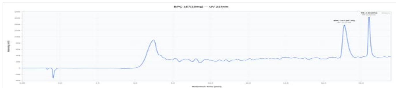
BPC-157 + TB-500 10mg - WV10-281: UV Chromatogram
