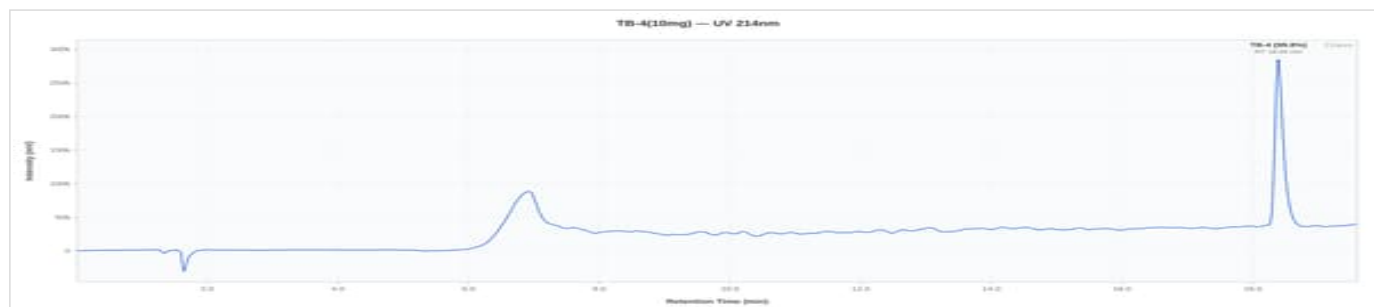
TB-500 10mg - TB10-262: UV Chromatogram
