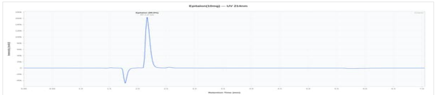
Epithalon 10mg - EP10-308: UV Chromatogram
