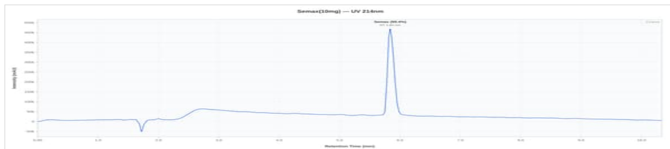
Semax 10mg - SMX10-274: UV Chromatogram
