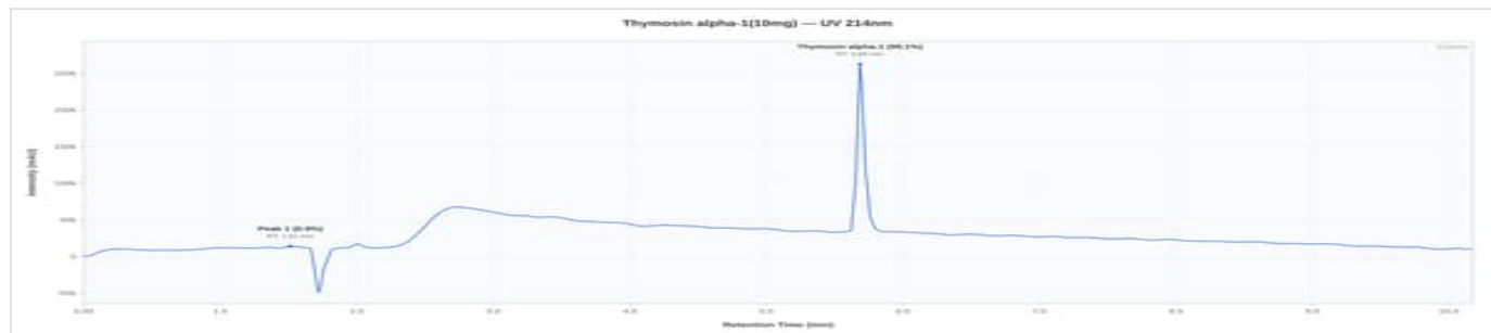
Thymosin Alpha-1 10mg - TA10-303: UV Chromatogram
